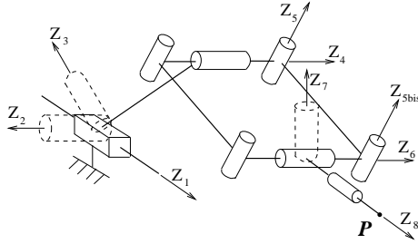
FIG. 5 – Flexible leg
