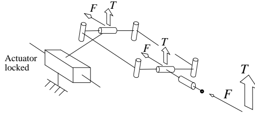
FIG. 4 – Forces transmitted in a leg
