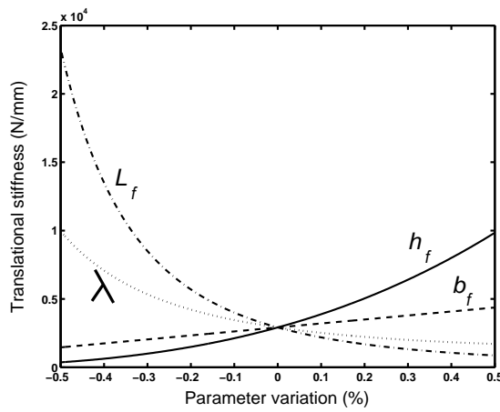
FIG. 7 – Quantitative influence of the geometric parameters h_f , b_f , L_f and d on the translational stiffness E = 2K_b
