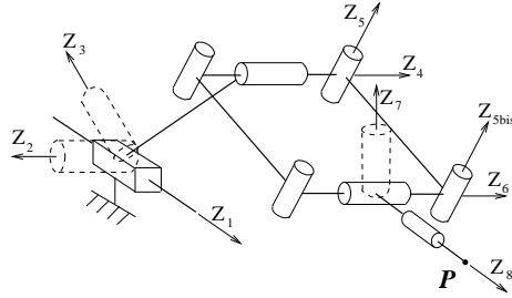
FIG. 5 – Flexible leg
