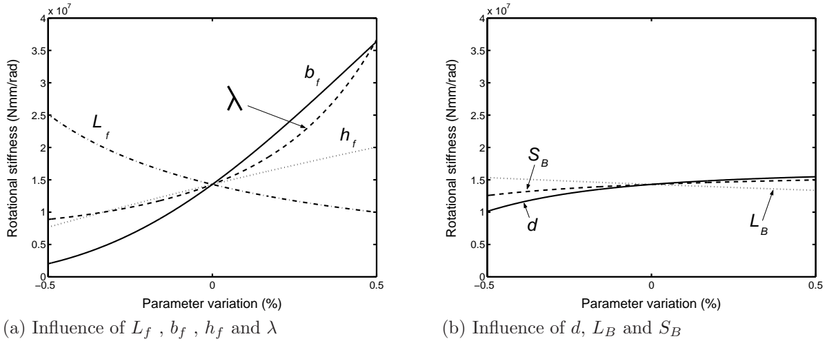
FIG. 6 – Quantitative influence of the geometric parameters on the rotational stiffness E = 2K_a
