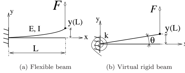
FIG. 3 – General model for flexible link
