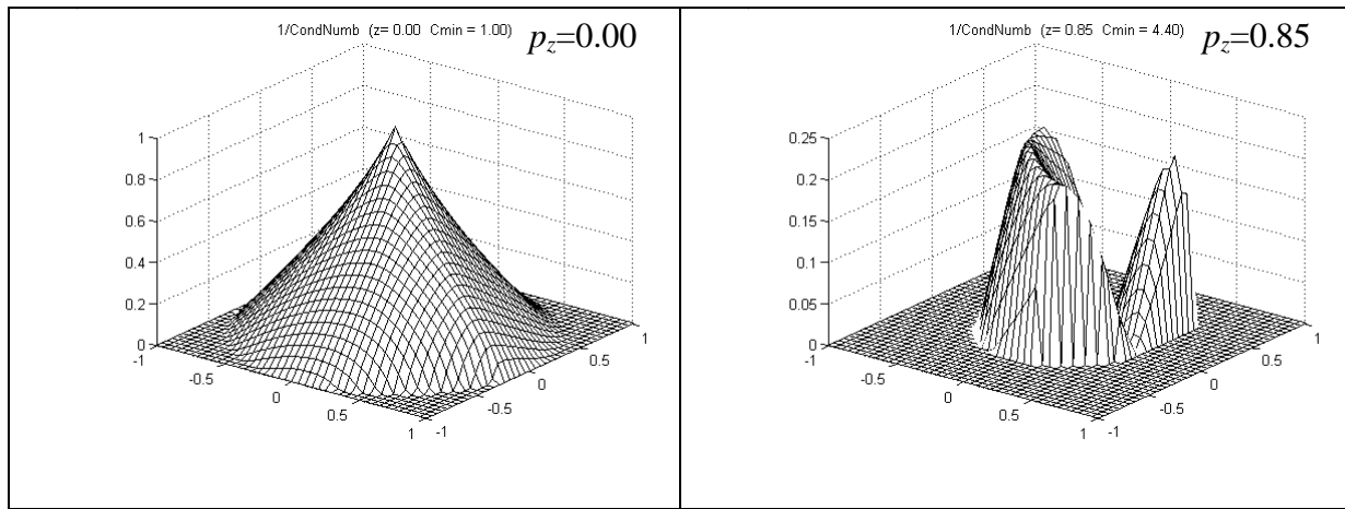
Fig. 15. Evolution of the cond(\mathbf{J})^{-1} for the horizontal sections.
