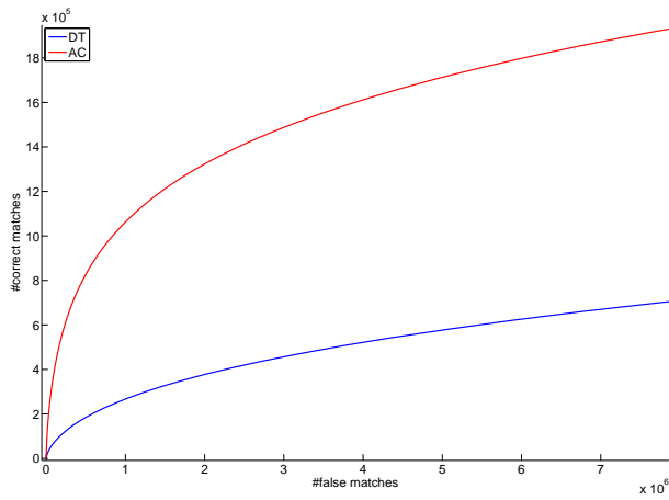
Fig. 8. Global ROC curves (on the whole database) for the A \rightarrow \{A' + A''\} protocol (the target is present twice, see Section (4.4)). Criterion AC is shown in red and criterion DT is shown in blue.
