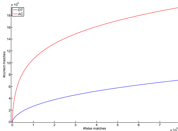
Fig. 8. Global ROC curves (on the whole database) for the A \rightarrow \{A'+A''\} protocol (the target is present twice, see Section (IV-D)). Criterion AC is shown in red and criterion DT is shown in blue.
