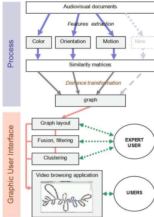
Fig. 1. The framework: a computing unit produces similarity matrices on video key frames, an expert user manipulates data and designs a profile to allow a video browsing in a collection.
