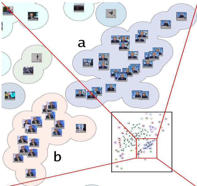
Fig. 3. Zoom of a layout applied on 161 frames of a newscast. The MDS algorithm uses a weighted normalized sum of color and orientation distances in order to improve the backbone clusters identification.
