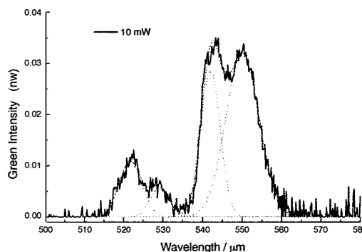
Fig.2 Green upconversion emission spectrum of an Er:ZBLALiP microsphere when pumped at 805 nm with 10 mw incident power.
