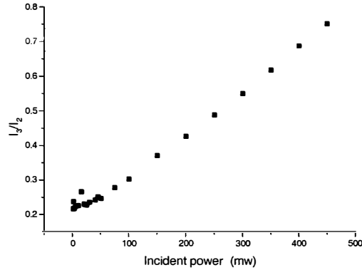
Fig.6 Dependence of the green emission intensity ratio on the incident pump power for the Er:ZBLALiP microsphere.
