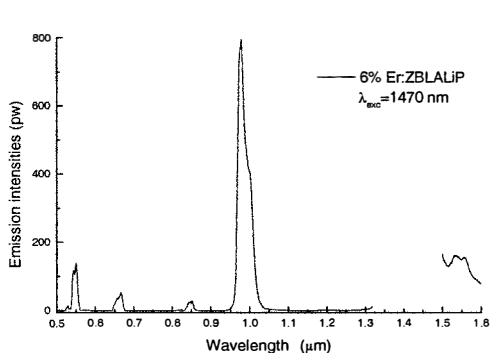
Fig.1 Upconversion emission spectrum of an Er:ZBLALiP when pumped at 1470 nm with 120 mw incident power.
