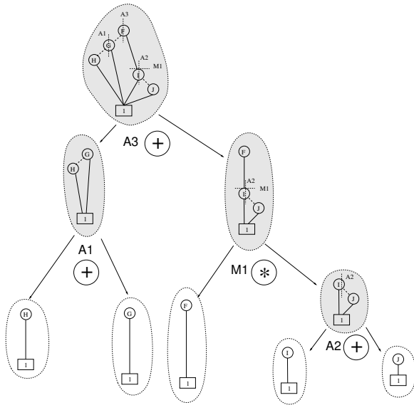
Fig. 5. Decomposition based on cut sequence (A3, M1, A2, A1) on TED for P in Figure 4.
