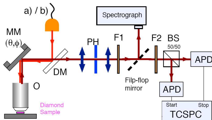
Figure 2. Experimental set-up. Excitation source: a) cw Ti:Sa laser tunable from 700 to 800 nm; b) picosecond pulsed laser emitting at 765 nm with 6 ps pulse duration and 20 MHz repetition rate; MM: Mobile mirror mounted on a scanning piezoelectric transducer; O: Microscope objective; DM: Dichroic mirror; PH: Pinhole with 100 \mu\text{m} diameter; F1: Long-pass interference filter transmitting wavelengths above 780 nm; F2: Band-pass filter centered at 800 nm and with a bandwidth of 10 nm FWHM; BS: non-polarized beamsplitter; APD: Silicon avalanche photodiode operated in photon counting regime; TCSPC: Time-correlated single-photon counting system (PicoHarp 300, PicoQuant, Germany); Spectrograph: Micro HR (Horiba Jobin Yvon, France) equipped with a CCD detector cooled at 200 K and a 1200 lines/mm grating blazed at 630 nm. The spectral resolution of the spectrograph is approximately 0.25 nm.
