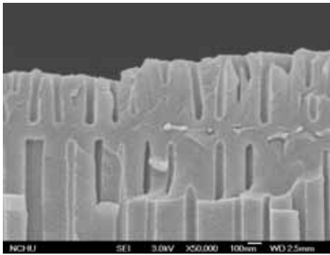
Figure 13. Cross-sectional image of the upper aluminum foil polished laminate
