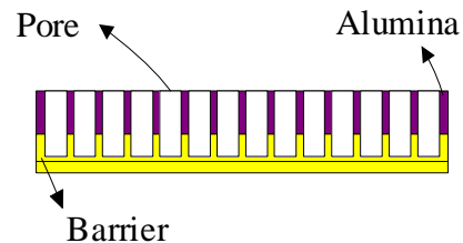
Figure 4. Anodized aluminum foils
