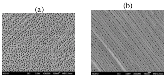
Top view of the upper foil Bottom view of the upper foil Figure 7. SEM images of the porous pattern of the unpolished aluminum laminate
