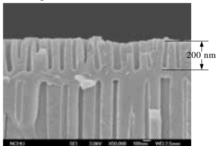
Figure 8. Cross-sectional image of the aluminum oxide of the unpolished laminate
