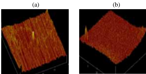
Figure 2. AFM image of the surface of (a) unpolished and (b) polished aluminum foils.
