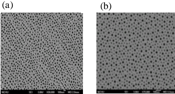
Figure 1. SEM image of the AAO made of (a) unpolished and (b) polished aluminum foils
