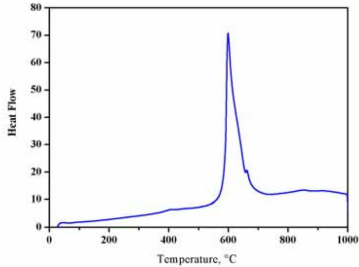
Fig.1. DTA trace of aluminum nanopowder.
