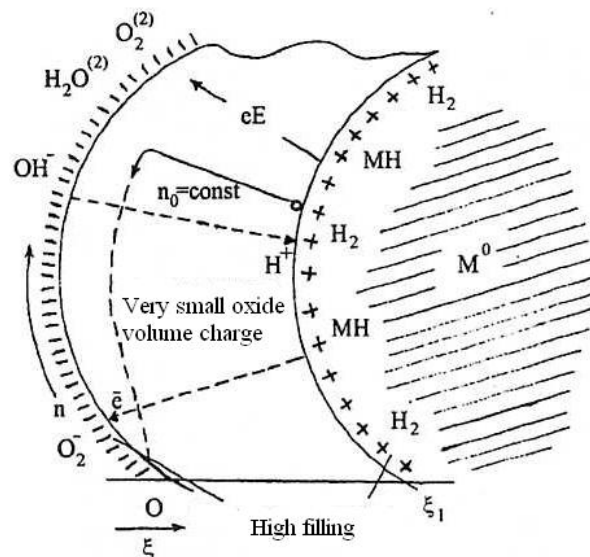
Fig.2. Scheme of the double electric layer in the nanosized particle.
