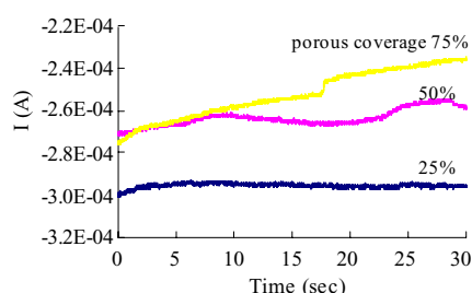
Figure 10. Dependence of the pumping property on the porous coverage
