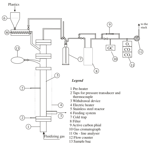
Figure 1. The bubbling fluidized bed reactor used for carrying out all the experiments
