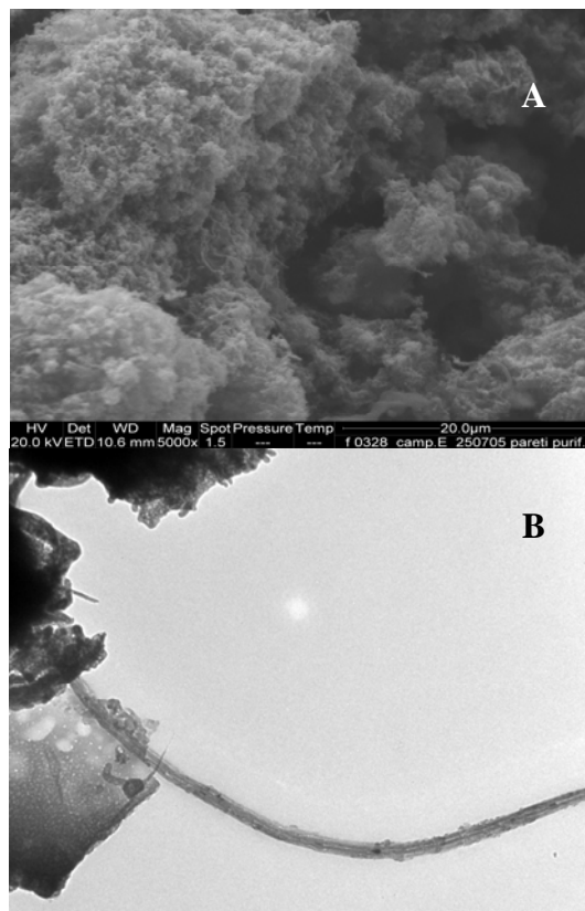
Figure 6. MWCNTs obtained after purification of samples produced with PP at 500°C: (A) SEM picture; (B)TEM picture.
