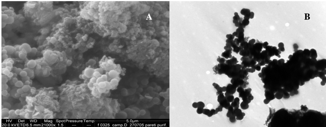
Figure 8. Nanotubes and other nanostructures obtained after purification of samples produced with PP at 700°C: (A) SEM picture; (B)TEM picture.
