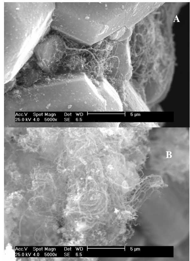
Figure 5 MWCNT agglomerates formed on the surface of bed particles in tests with PP in a bed of alumina.
