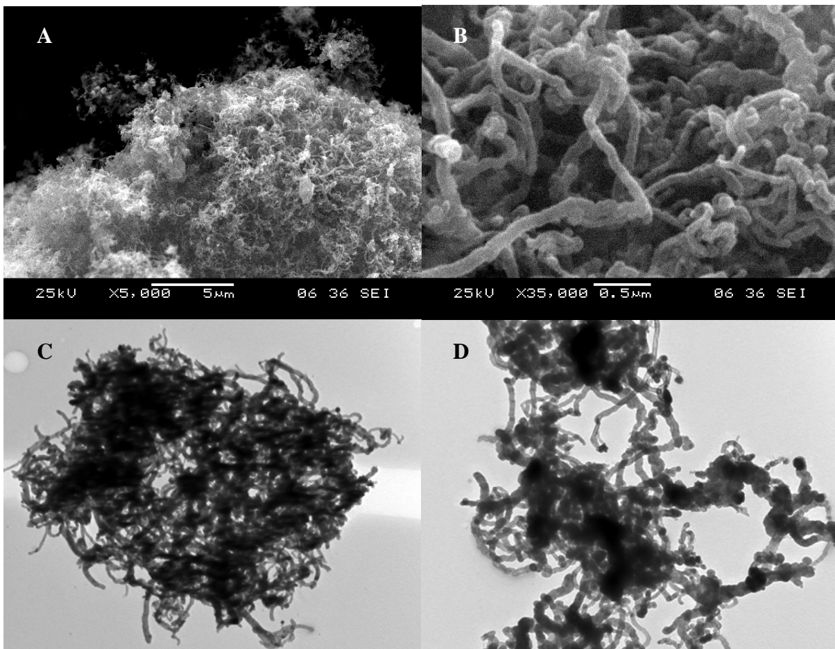
Figure 9 MWCNTs obtained with PET at 600°C: (A-B) SEM pictures of not purified samples; (C-D) TEM pictures of purified samples.
