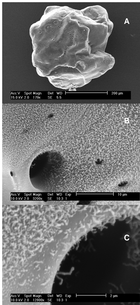
Figure 2 Scanning electronic pictures of MWCNTs as obtained in a test with PET. (A) A bed particle covered by a thin layer of polymer; (B and C) Details of the polymer layer.
