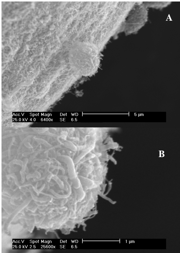
Figure 4 MWCNT agglomerates formed on the surface of bed particles in tests with PP in a bed of quartz sand.
