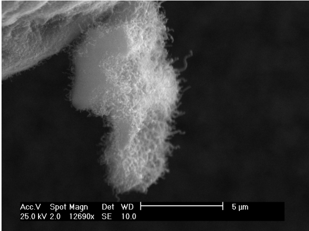
Figure 3 SEM picture of MWCNT agglomerate at the surface of a bed particle in a test with PET.
