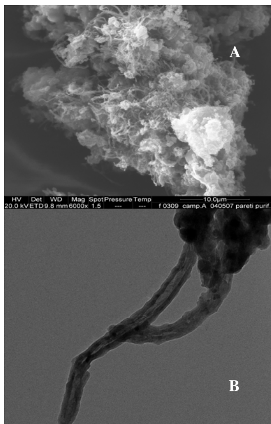
Figure 7 MWCNTs obtained after purification of samples produced with PP at 600°C: (A) SEM picture; (B)TEM picture.
