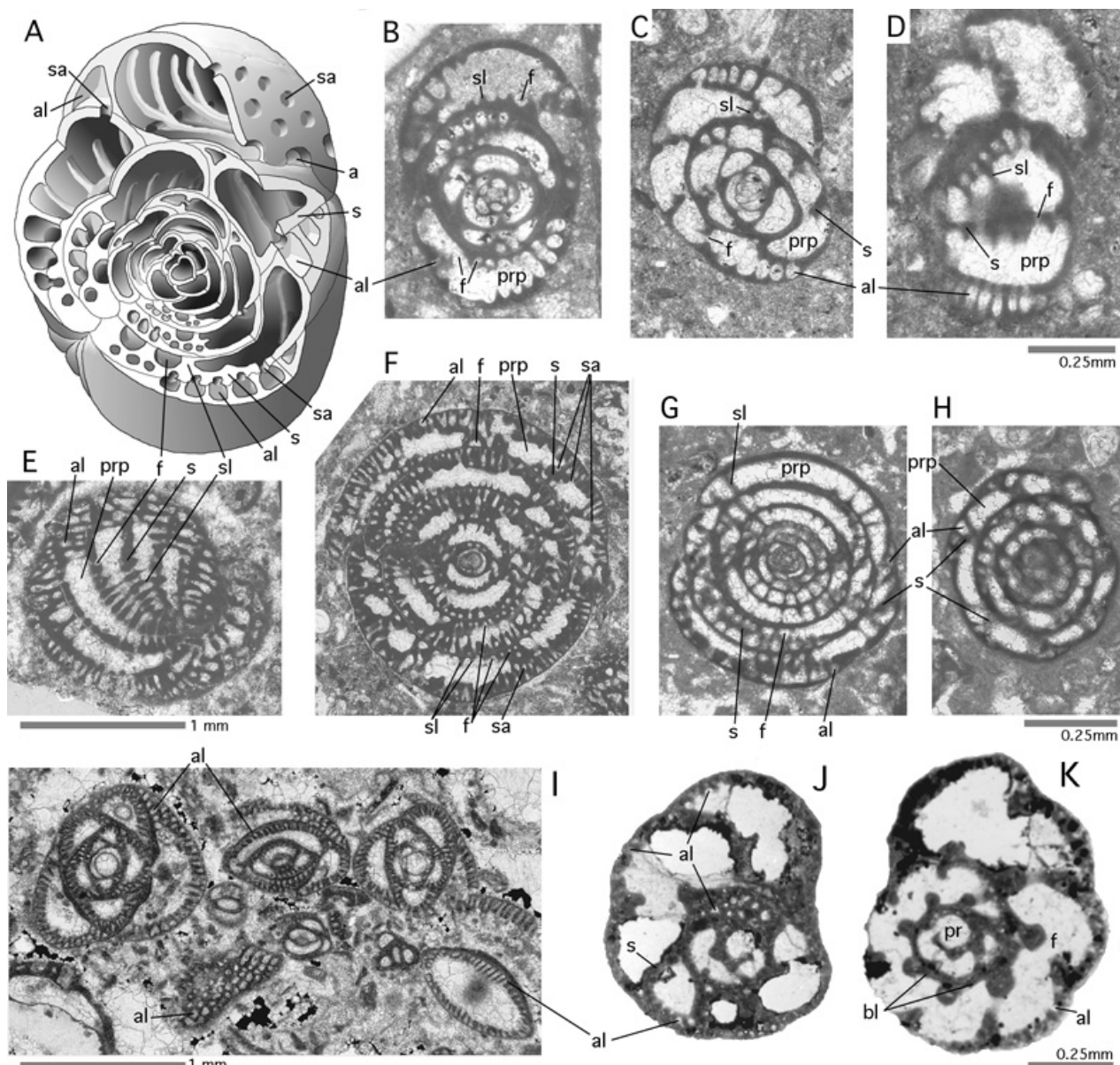
Figure 9: Alveoles.
