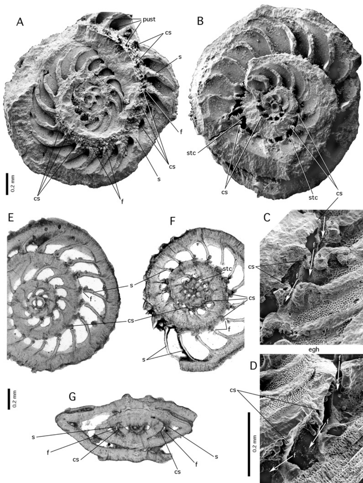
Figure 33: Countersepta.
