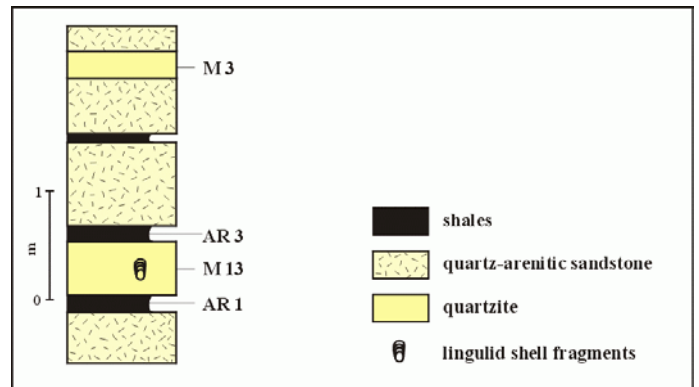
Figure 4: Schematic lithostratigraphy of the section sampled.
