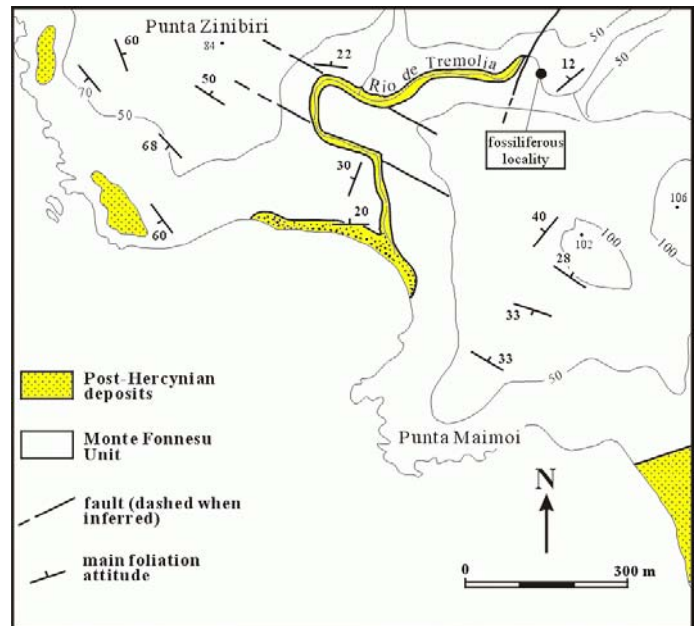
Figure 3: Geologic sketch map of the area studied.
