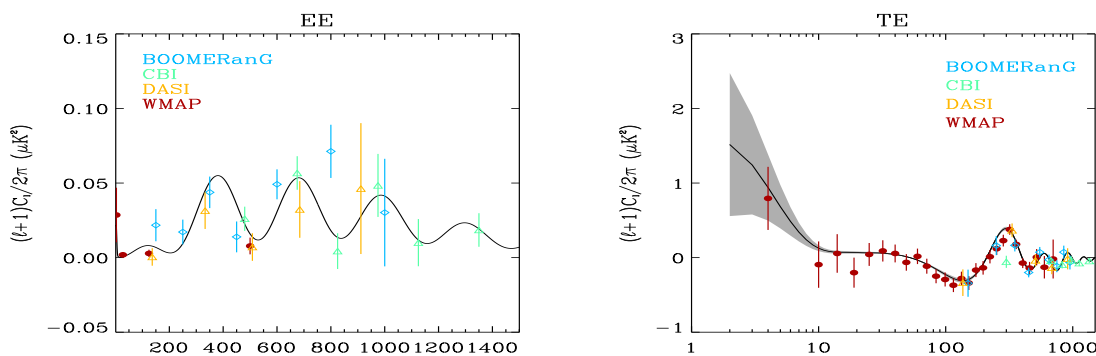
Figure 21. E-mode spectrum (left) and TE (right) measured by BOOMERanG [Montroy et al (2006), Piacentini et al (2006)], DASI [Leitch et al (2005)], CBI [Readhead et al (2004)] and WMAP [Page et al (2006), Hinshaw et al (2006)].
