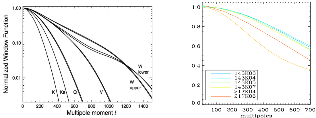
Figure 16. Beam window function in multipole space for a WMAP ( left , extracted from LAMBDA, http://lambda.gsfc.nasa.gov ) detector, and Archeops ( right , extracted from [Tristram et al (2005b)])
