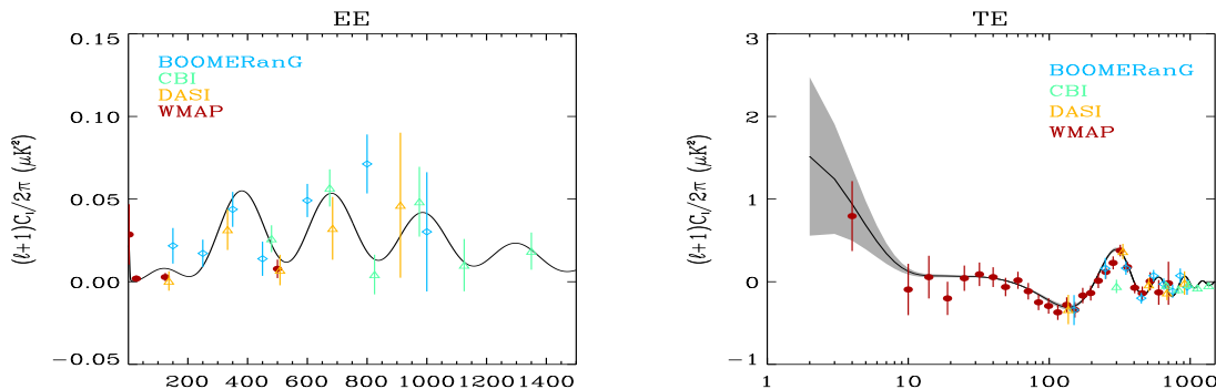
Figure 21. E-mode spectrum ( left ) and TE ( right ) measured by BOOMERanG [Montroy et al (2006), Piacentini et al (2006)], DASI [Leitch et al (2005)], CBI [Readhead et al (2004)] and WMAP [Page et al (2006), Hinshaw et al (2006)].
