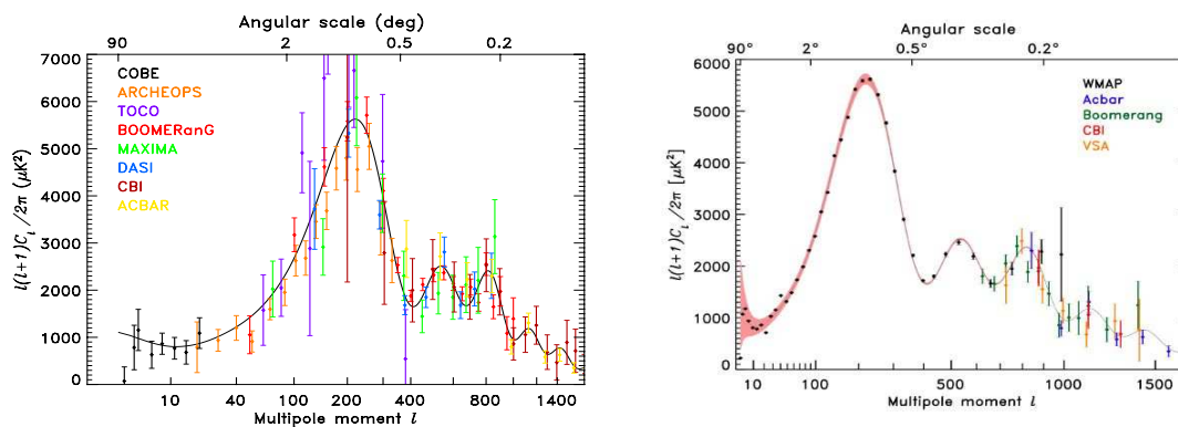
Figure 20. Left: CMB temperature angular power spectrum before WMAP in 2003 (COBE [Tegmark (1996a)], Archeops [Benoit et al (2003)], TOCO [Miller et al (2002)], BOOMERanG98 [Ruhl et al (2003)], Maxima01 [Lee et al (2001)], DASI [Halverson et al (2002)], CBI [Pearson et al (2003)] and ACBAR [Kuo et al (2004)]). (extracted from [Hinshaw et al (2003)]) Right: Results from the 3 years observation of WMAP [Hinshaw et al (2006)] together with last results from high resolution experiments: BOOMERanG [Jones et al (2006)], Acbar [Kuo et al (2004)], CBI [Readhead et al (2004)] and VSA [Dickinson et al (2004)]. (extracted from [Hinshaw et al (2006)])
