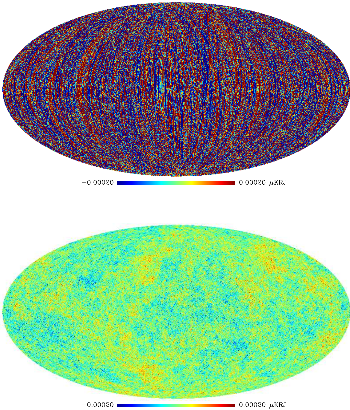
Figure 19. Simulation at 217 GHz for Planck before ( top ) and after destripping ( bottom ). Simulations only include 1/f noise and CMB signal.
