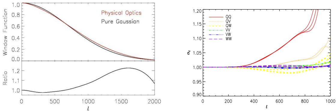
Figure 17. Effects of beam asymmetry on C_\ell . Left: for a BOOMERanG bolometer at 145 GHz, computed from the physical optics model (red line) and a 9.8 arcmin FWHM gaussian beam (black line). (figure extracted from [Masi et al (2006)]) Right: ratio between the window function for the actual beam and that for a gaussian beam for each WMAP channel. (Figure extracted from [Hinshaw et al (2006)])
