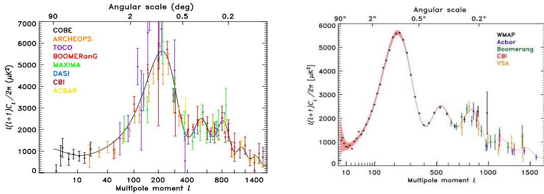
Figure 20. Left: CMB temperature angular power spectrum before WMAP in 2003 (COBE [Tegmark (1996a)], Archeops [Benoît et al (2003)], TOCO [Miller et al (2002)], BOOMERanG98 [Ruhl et al (2003)], Maxima01 [Lee et al (2001)], DASI [Halverson et al (2002)], CBI [Pearson et al (2003)] and ACBAR [Kuo et al (2004)]). (extracted from [Hinshaw et al (2003)]) Right: Results from the 3 years observation of WMAP [Hinshaw et al (2006)] together with last results from high resolution experiments: BOOMERanG [Jones et al (2006)], Acbar [Kuo et al (2004)], CBI [Readhead et al (2004)] and VSA [Dickinson et al (2004)]. (extracted from [Hinshaw et al (2006)])
