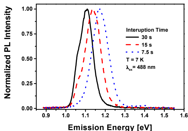
Fig. 2. Normalised PL spectra of single QD structures prepared with different growth interruption time measured at 7 K. TEM image of three InAs QD layers sample with 3.7 nm thick separation GaAs layer.
