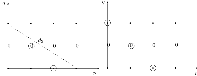
FIGURE 2. Terms E_3^{pq}(\mathcal{X}) and E_4^{pq}(\mathcal{X})
