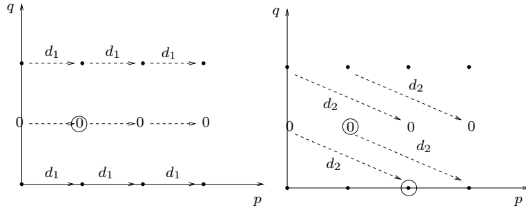
FIGURE 1. Terms E_1^{pq}(\mathcal{X}) and E_2^{pq}(\mathcal{X})
