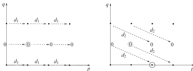
Figure 1. Terms E_1^{pq}(\mathcal{X}) and E_2^{pq}(\mathcal{X})
