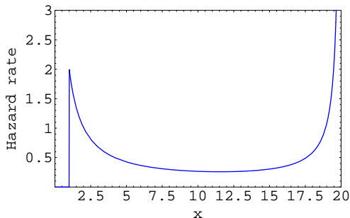
Fig. 5. Hazard rate h(x) for the upper bounded Pareto distribution with parameters k = 1 , p = 20 , \alpha = 2 .
