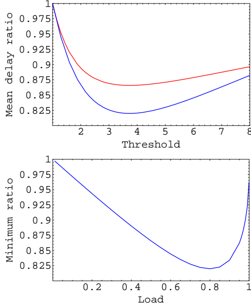
Fig. 3. Pareto distribution with parameters k = 1 , \alpha = 2 . Top : Mean delay ratio \overline{T}^{\text{FCFS+FB}(\theta)}/\overline{T}^{\text{FB}} as a function of threshold \theta for loads \rho = 0.5 (upper curve) and \rho = 0.8 (lower curve). Bottom : Minimum mean delay ratio \overline{T}^{\text{FCFS+FB}(\theta^*)}/\overline{T}^{\text{FB}} as a function of load \rho .
