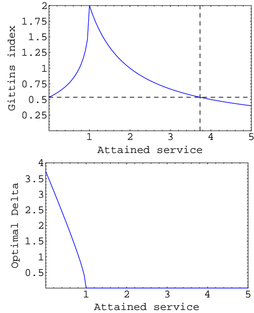
Fig. 2. Pareto distribution with parameters k = 1 , \alpha = 2 . Top: Gittins index G(a) as a function of attained service a with the horizontal dashed line equal to G(0) and the vertical dashed line equal to a = \Delta^*(0) . Bottom: Optimal \Delta^*(a) as a function of attained service a .
