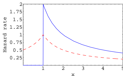
Fig. 1. Functions h(x) (solid curve) and H(x) (dashed curve) for the Pareto distribution with parameters k = 1 , \alpha = 2 .
