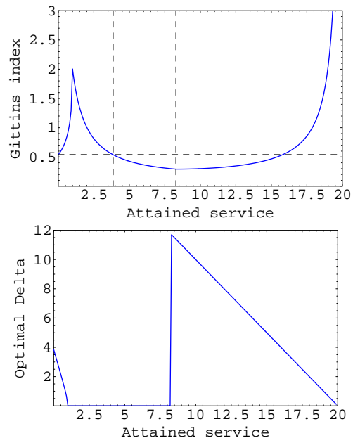
Fig. 6. Upper bounded Pareto distribution with parameters k = 1 , p = 20 , \alpha = 2 . Top : Gittins index G(a) as a function of attained service a with the horizontal dashed line equal to G(0) and the two dashed vertical lines equal to a = \Delta^*(0) = 3.855 and a = 8.284 , respectively. Bottom : Optimal \Delta^*(a) as a function of attained service a .
