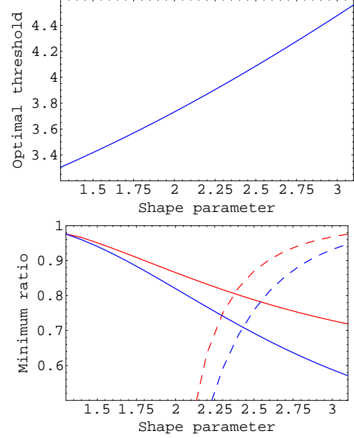
Fig. 4. Pareto distributions with parameters fixed k = 1 and varying \alpha . Top : Optimal threshold \theta^* = \Delta^*(0) as a function of \alpha . Bottom : Minimum mean delay ratios \overline{T}^{\text{FCFS+FB}(\theta^*)}/\overline{T}^{\text{FB}} (solid lines) and \overline{T}^{\text{FCFS+FB}(\theta^*)}/\overline{T}^{\text{FCFS}} (dashed lines) as a function of \alpha for loads \rho = 0.5 (upper curves) and \rho = 0.8 (lower curves).
