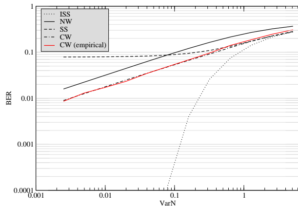
Figure 8: Comparison of BER for NW, classical SS, ISS and CW-ISS. N_v = 512 , WCR = -21dB and N_c = 2 .
