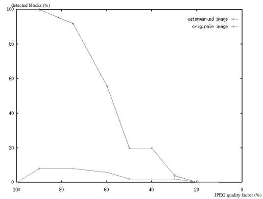
Figure 7: JPEG-test with the spatial scheme
