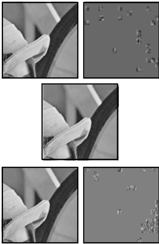
Figure 8: In the upper part: the watermarked image and the added information (rescaled) using our DCT algorithm, in the lower part: the watermarked image and the added information (rescaled) using our spatial algorithm, in the middle part: the original image
