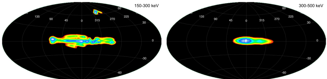
FIGURE 2. Point-source subtracted INTEGRAL/SPI multiresolution maps in the energy bands 150-300 keV (left) and 300-500 keV (right).
