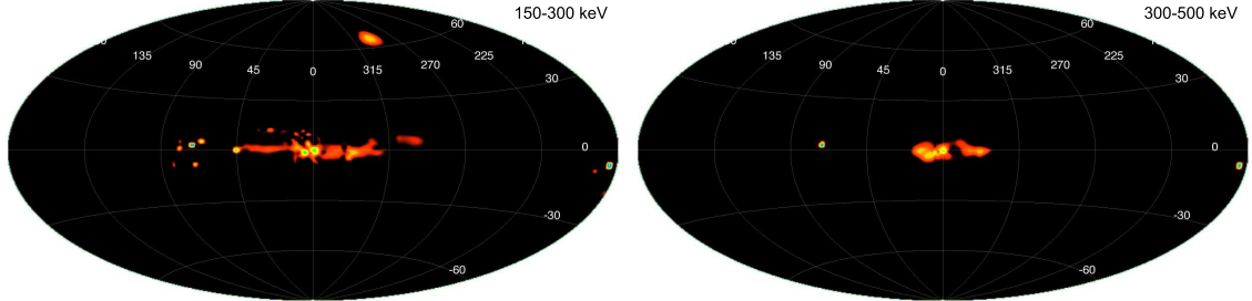
FIGURE 1. INTEGRAL/SPI multiresolution maps in the energy bands 150-300 keV (left) and 300-500 keV (right).
