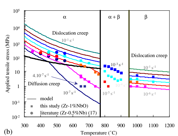
Fig. 5. Deformation-mechanism maps for (a) Zy-4 and (b) Zr-1%NbO. Lines of constant true axial strain rate are plotted using the model presented in this paper.
