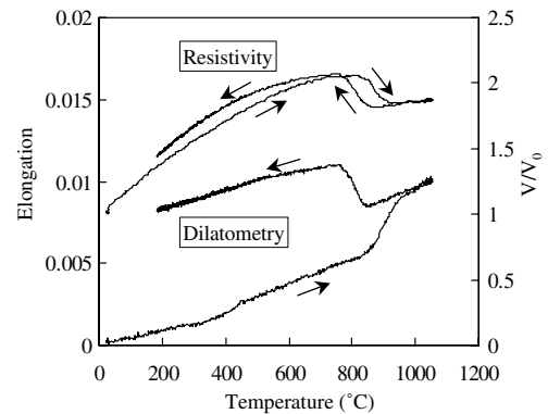
Fig. 1. Resistivity and dilatometry curves (Zr-1%NbO, 50 ^{\circ}\text{C}/\text{min} ). V is the DC potential, of initial value V_0 .
