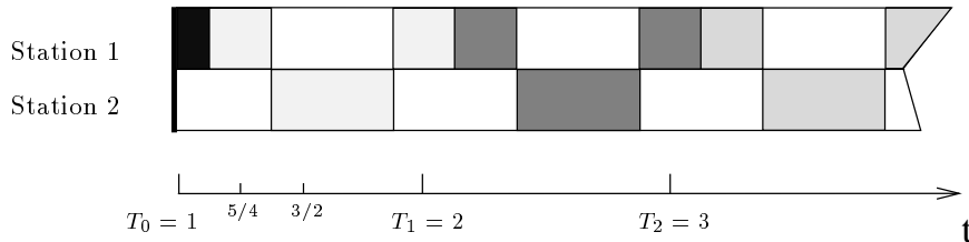
FIG. 2. Initial condition (Q^1, R^1) = (1, 9/8), (Q^2, R^2) = (0, 0) .
