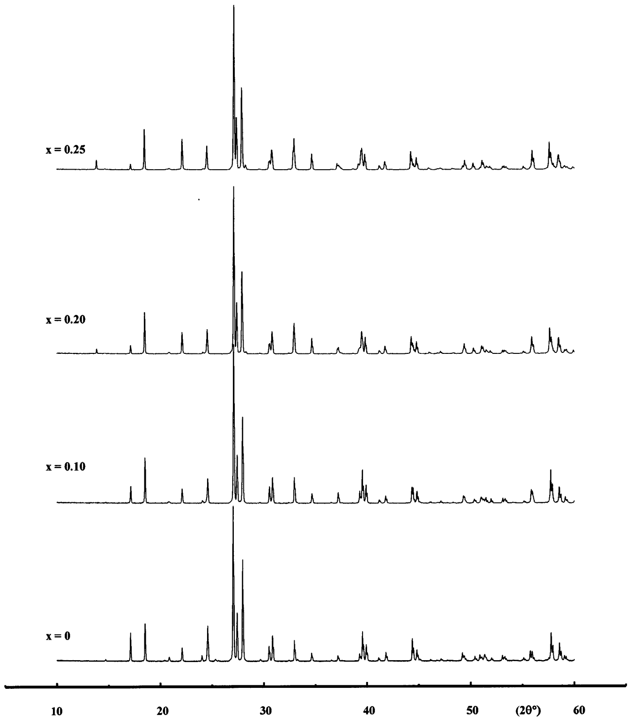
Figure 1. X-ray powder diffraction patterns of \text{Li}_{(1-2x)}\text{Ni}_x\text{TiO}(\text{PO}_4) ( x=0;0.10;0.20;0.25 ).
