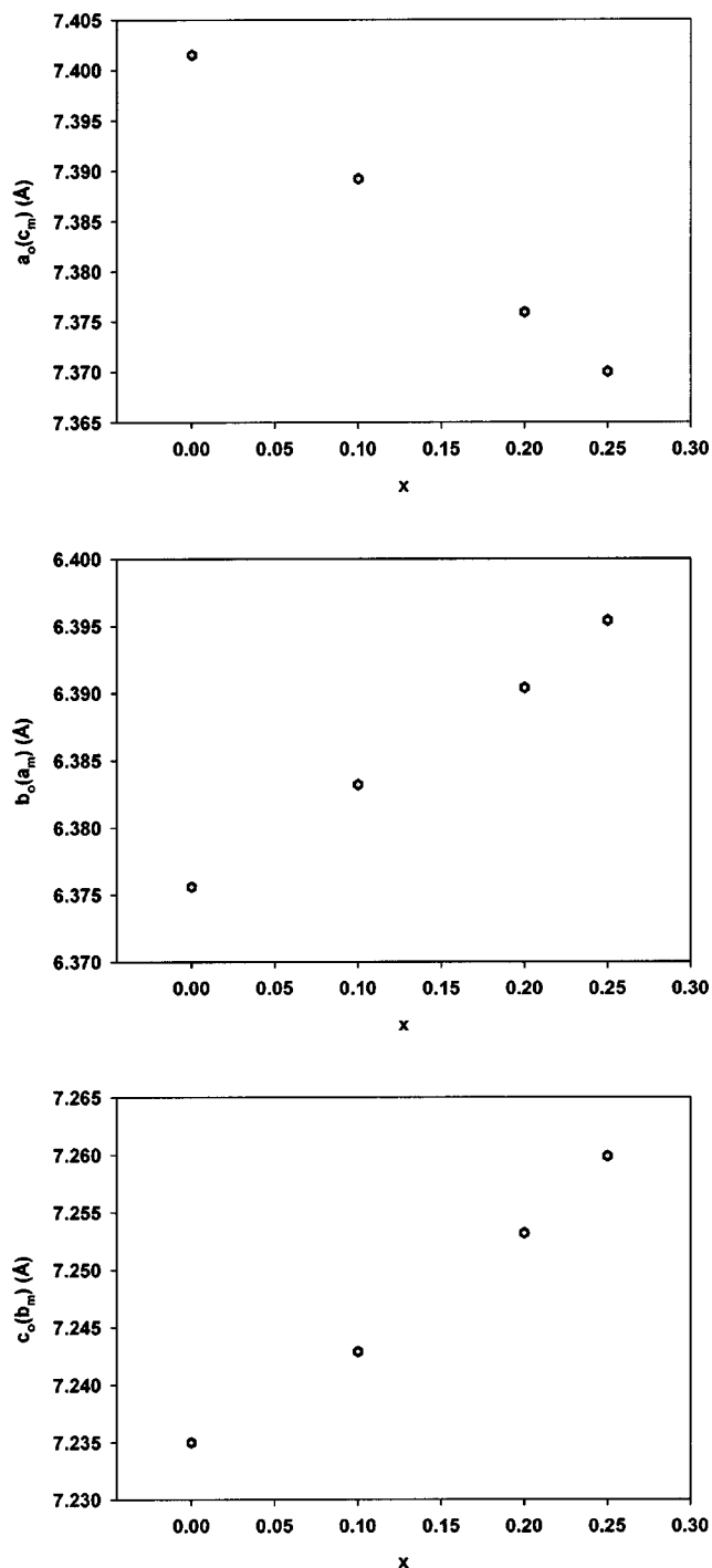
Figure 2. Cell parameter variations as a function of x for \text{Li}_{(1-2x)}\text{Ni}_x\text{TiO}(\text{PO}_4) ( 0 \leq x \leq 0.25 ), where progressive substitution of lithium by nickel provokes a decrease of a_o(c_m) and an increase of b_o(a_m) and c_o(b_m) .
