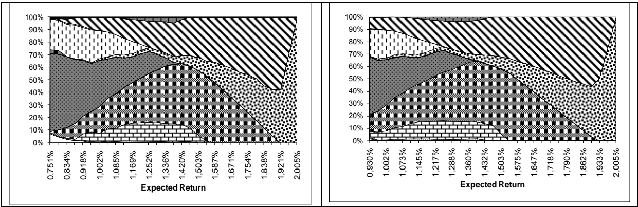
Fig 3-6: Efficient allocations for Fischer measure (a=85%)(left) and Denneberg absolute deviation (right)(a=85%)
