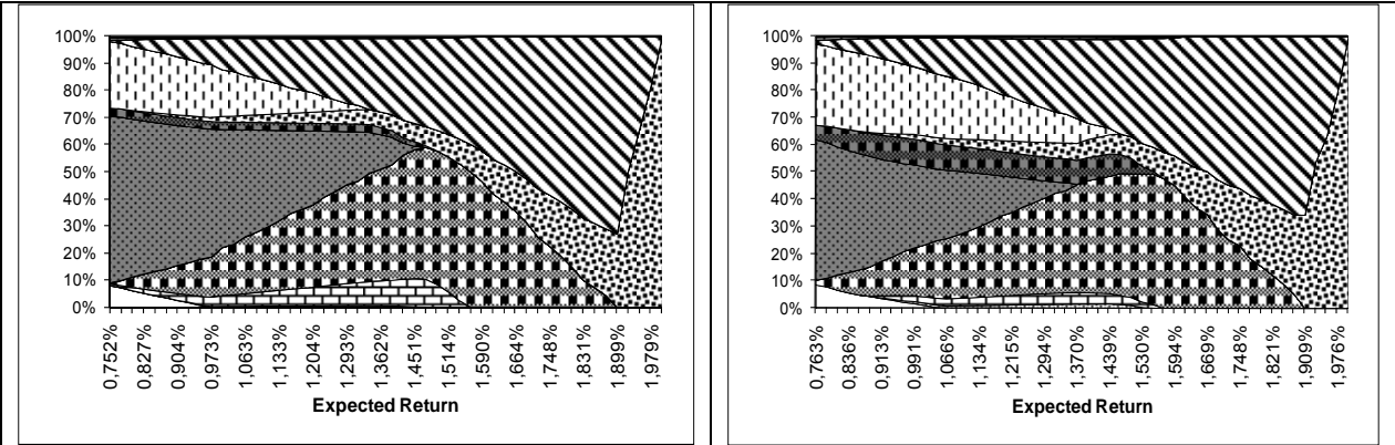
Fig 3-5: Efficient allocations for standard deviation (left) and lower semi-variance (right)
