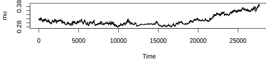
Fig. 15. Evolution of \mu[1 + n..25000 + n] for n = 0, 1, 2, \dots
