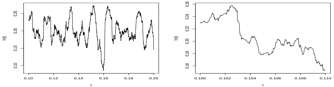
Fig. 13. Evolution of the estimated H(t) on [0.1, 0.2] and [0.1, 0.11]
