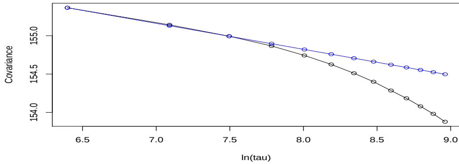
Fig. 14. Autocorrelation function and logarithmic decrease
