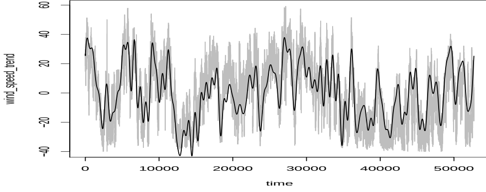
Fig. 11. Trend on 72 harmonics
