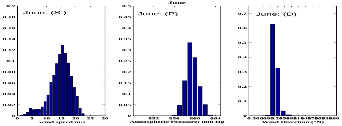
Fig. 4. Densities of (S,P,D) in June 2004
