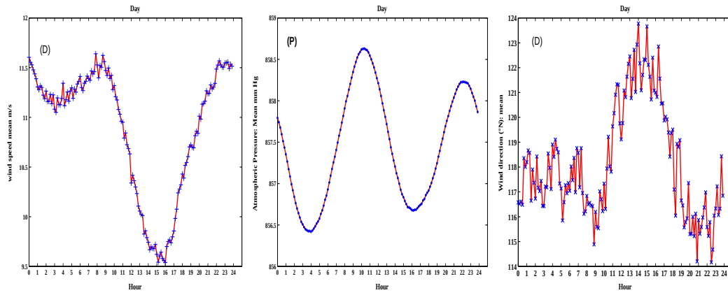
Fig. 6. Average Day profile of (S,P,D) for 2004.
