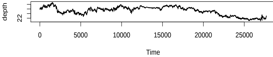
Fig. 17. Levels of cascades [1+n..25000+n] for n = 0, 1, 2, \dots
