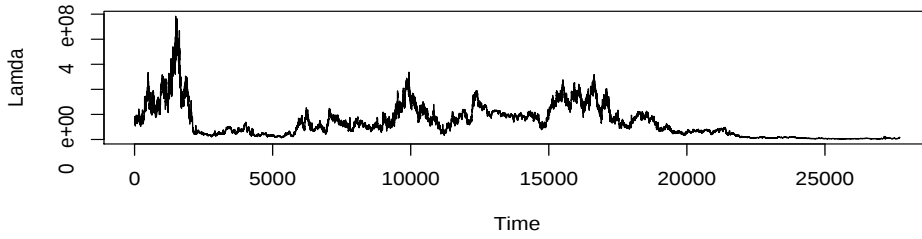
Fig. 16. Evolution of \lambda[1 + n..25000 + n] for n = 0, 1, 2, \dots
