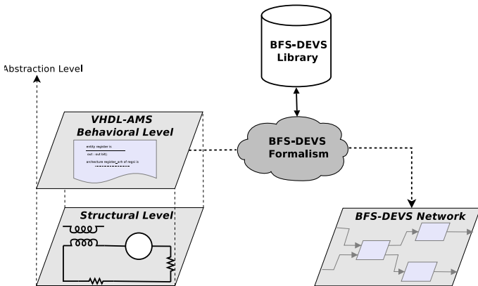
Fig. 6. BFS-DEVS for VHDL circuit modelling
