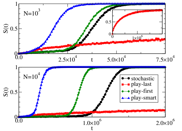
FIG. 9: Success rate curves S(t) for the various strategies: stochastic, "play-last", "play-first" and "play-smart". At the beginning of the process the stochastic and "play-first" strategies yield similar success rates, but then the deterministic rule speeds up convergence. On the other hand also the "play-smart" and the "play last" evolve similarly at the beginning, but the latter reaches the final state much earlier through a steep jump. It is worth noting that for three strategies the S(t) curves present a characteristic S -shaped behavior, while in the "play-last" one the disorder-order transition is more continuous (see inset in the top figure). All curves, both for N = 10^3 and N = 10^4 , have been generated averaging over 3 \times 10^3 simulation runs.
