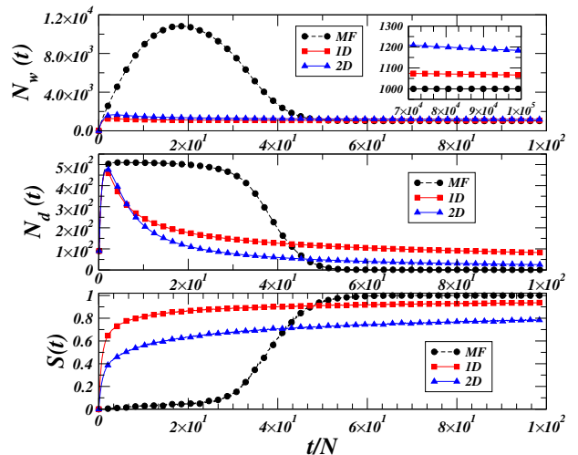
FIG. 2: Evolution of the total number of words N_w (top), of the number of different words N_d (center), and of the average success rate S(t) (bottom), for a mean-field system (black circles) and low-dimensional lattices (1D, red squares and 2D, blue triangles) with N = 1024 agents, averaged over 10^3 realizations. The inset in the top graph shows the very slow convergence in low-dimensional lattices.
