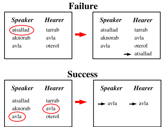
FIG. 1: Agents interaction rules. Each agent is described by its inventory, i.e. the repertoire of known words. The speaker picks up at random a name in its inventory and transmits it to the hearer. If the hearer does not know the selected word the interaction is a failure (top), and it adds the new name to its inventory. Otherwise (bottom), the interaction is a success and both agents delete all their words but the winning one. Note that if the speaker has an empty inventory (as it happens at the beginning of the game), it invents a new name and the interaction is a failure.
