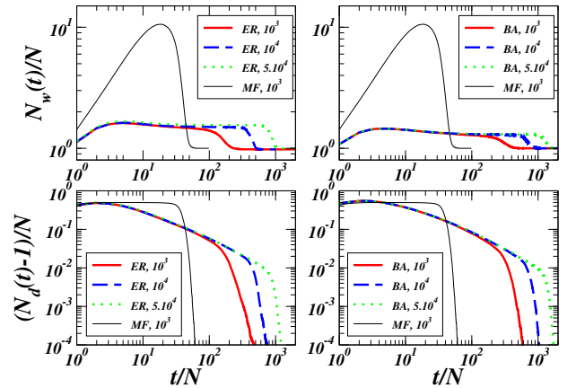
FIG. 5: ER random graph (left) and BA scale-free network (right) with \langle k \rangle = 4 and sizes N = 10^3, 10^4, 5 \cdot 10^4 . Top: evolution of the average memory per agent N_w/N versus rescaled time t/N . For increasing sizes a plateau develops in the re-organization phase preceding the convergence. The height of the peak and of the plateau collapse in this plot, showing that the total memory used scales with N . Bottom: evolution of the number of different words N_d in the system. (N_d - 1)/N is plotted in order to emphasize the convergence to the consensus with N_d = 1 . A steady decrease is observed even if the memory N_w displays a plateau. The mean-field (MF) case is also shown (for N = 10^3 ) for comparison.
