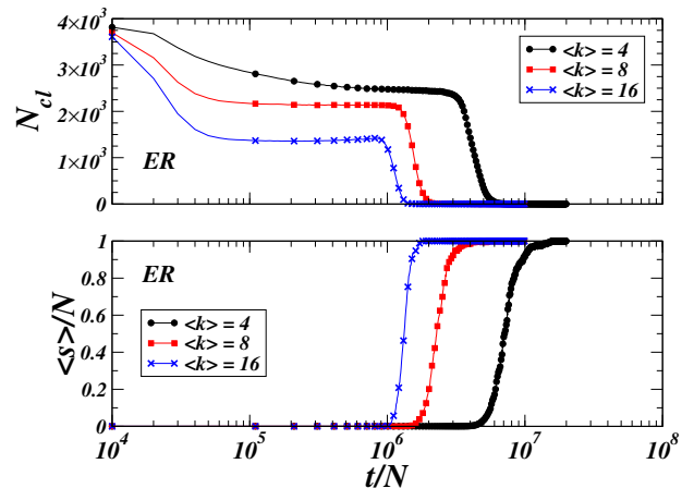
FIG. 7: Number of clusters N_{cl} and normalized average cluster size \langle s \rangle/N vs. time for ER networks with N = 10^4 , \langle k \rangle = 4 (circles), \langle k \rangle = 8 (squares), \langle k \rangle = 16 (crosses).
