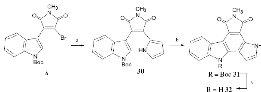
Scheme 2. Reagents and conditions: (a) pyrrolyl-MgBr (3 equiv), THF, rt, 24 h (78% yield); (b) halogen lamp (500 W), \text{CH}_3\text{CN} , rt, 31 h (87% yield); (c) \text{HCOOH} , rt, 16 h (76% yield).
