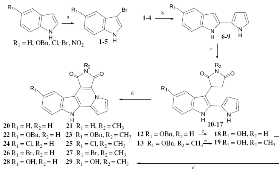
Scheme 1. Reagents and conditions: (a) \text{Br}_2 (1 equiv), DMF, rt or 0 ^\circ\text{C} , 12 h (61–92% yield); (b) pyrrole (1 equiv), TFA, \text{CH}_2\text{Cl}_2 (67–72% yield); (c) maleimide or N -methylmaleimide (2 equiv), \text{SnCl}_2 catalytic, toluene, reflux (46–96% yield); (d) Pd black, nitrobenzene, 200 ^\circ\text{C} , 4–8 h (16–92%); (e) Pd/C, EtOAc/MeOH 1:2, \text{H}_2 1 bar 12–24 h (89–100%).
