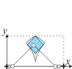
Figure 13: The Cartesian workspace of the Biglide1
