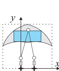
Figure 14: The Cartesian workspace of the Biglide2
