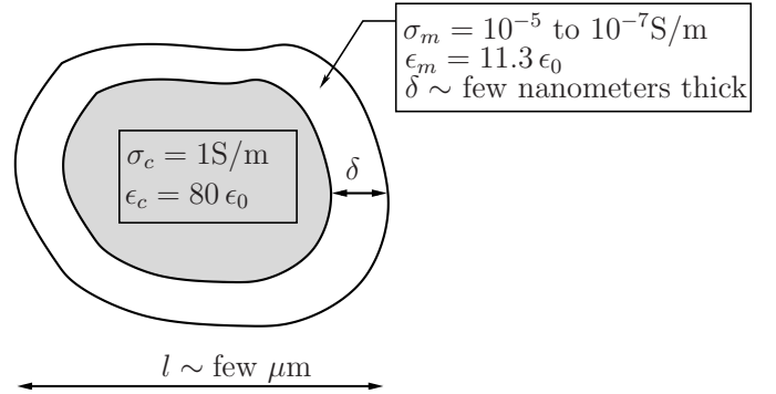
Fig. 1. The electric model of the biological cell (see Fear et al. [5]).
