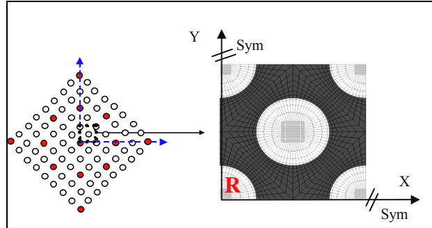
Figure 6: Example of a Representative Elementary Volume of a damage state and geometry of the Periodic Elementary Cell (the red circles and R represent the broken fibres)
