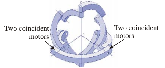
Figure 9: Redundant spherical wrist
