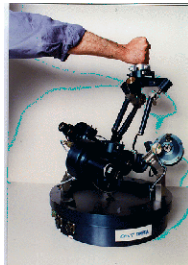
Figure 2: The “syntaxeur” from ONERA/CERT [3]
