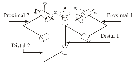
Figure 10: The hybrid agile eye with two-dof in serial with a revolute actuated joint 3
