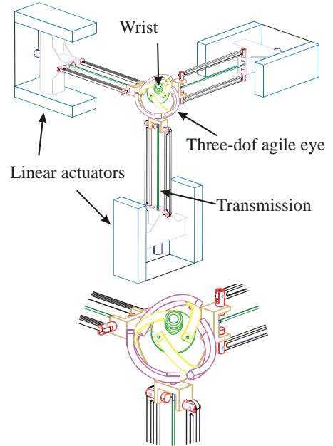
Figure 13: A six-dof haptic device 3T+3R
