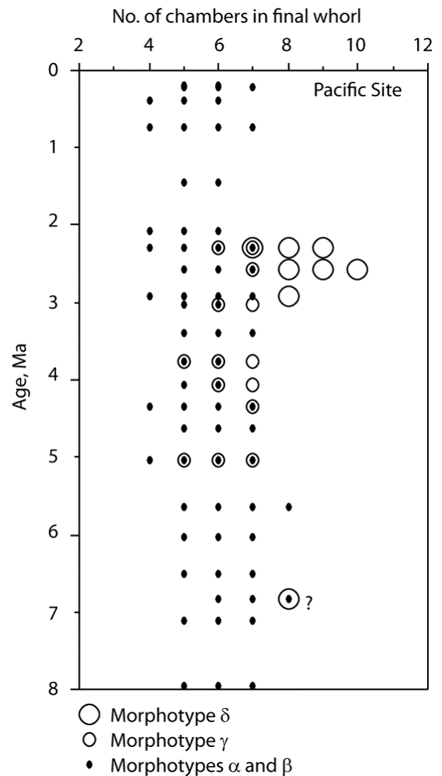
Figure 15: Number of chambers in the final whorl of morphotypes alpha and beta , morphotypes gamma and delta over time at DSDP Site 503 and 503A. Symbols as in Figure 14.
