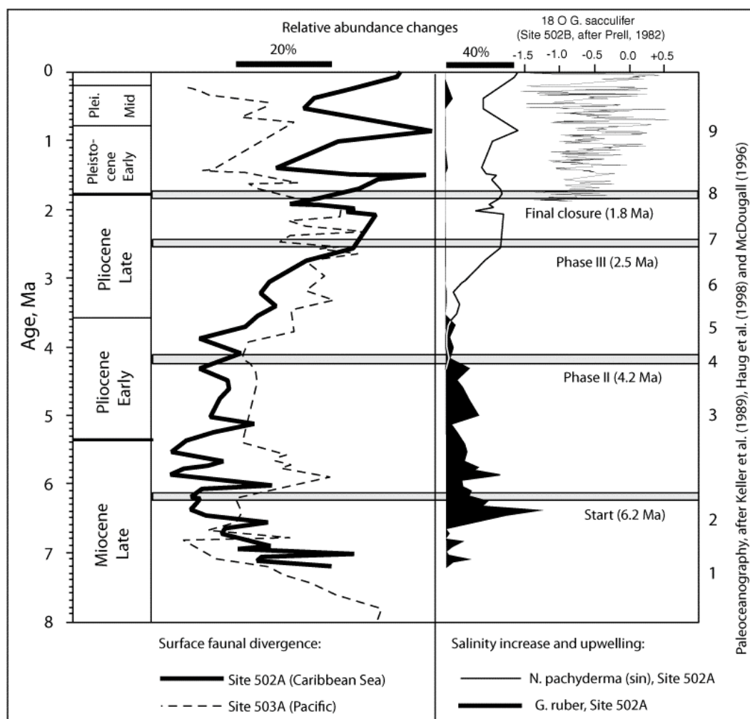
Figure 3: Palaeoceanographic summary of the emergence of the Isthmus of Panama (after KELLER et alii , 1989; MCDUGALL, 1996; HAUG et alii , 1998). Numbers on the right margin of the diagram concern palaeoceanographic events: 1). Benthic and planktic faunal provinces on either side of the ancient Central American seaway are similar (until 6.7 Ma (Caribbean) and 6.2 Ma (Pacific)). Before 5.6Ma: North Atlantic Deep Water (NADW) flowed across a rising sill into the Pacific. After 5.6 Ma: Deep water flows across the sill ended; 2). Before 4.6–4.5 Ma: Poor ventilation in the Caribbean and dissolution of the carbonate skeletons of plankton. Onset of upwelling in the Caribbean, disruption of intermediate water flow to Pacific. Siliceous microfossils are absent in sediments younger than 6 Ma; 3). Major upwelling in Caribbean; 4). Onset of increased salinity in the surface water of the Caribbean (4.6–4.2 Ma); 5). Increasing abundance of surface water species tolerant of high salinity; 6). Major intensification of Northern Hemisphere glaciation (3.3–2.9 Ma); 7). Permanent isolation of faunal provinces (drop in sea level, connection between Atlantic and Pacific very restricted); 8). Permanent closure of the seaway across the Isthmus of Panama, continued increase in the divergence of the assemblages of surface-dwelling plankton of the Pacific and Caribbean; 9). Major increase in the salinity of the Caribbean Sea. Pleistocene, right-hand column: Oxygen isotope curve for Globigerinoides sacculifer at DSDP Site 502B (PRELL, 1982).
