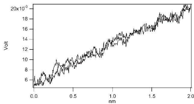
Figure 7 Lateral force – lateral displacement cycle for a cured film of thickness of about 1 \mu\text{m} with a DH/TH ratio equal to 0.98, obtained with a scan perpendicular to the axis of the cantilever at a frequency of 2 Hz and at zero normal load.
