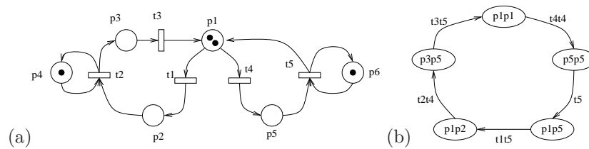
Figure 7: Free-choice net and its worst evolution.
