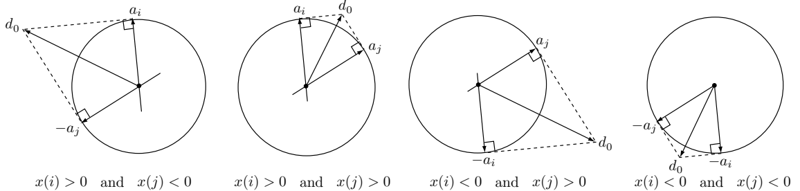
Figure 1: Four different configurations of coefficients (x_0(i), x_0(j)) and the corresponding d_0 .
