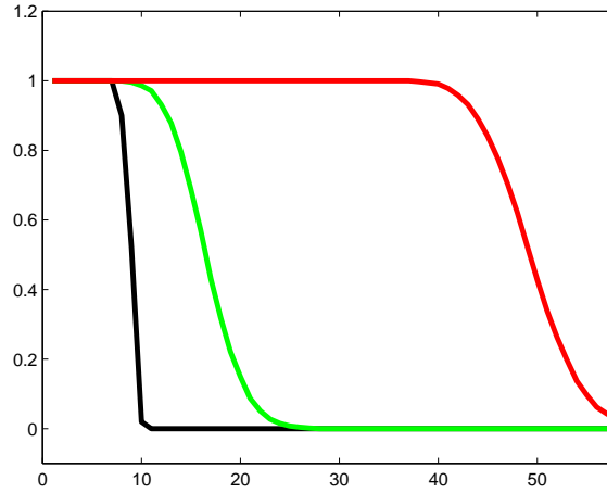
Figure 9: Proportions of vectors satisfying each of the three criteria ERC > 0 , F < 1 and F^+ < 1 as a function of sparsity d . The black line corresponds to the condition ERC > 0 , the green line to F < 1 and the red one to F^+ < 1 .
