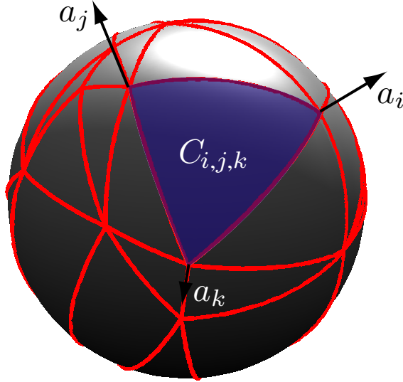
Figure 7: Example of a cone C_{i,j,k} belonging to the set \mathcal{T} .
