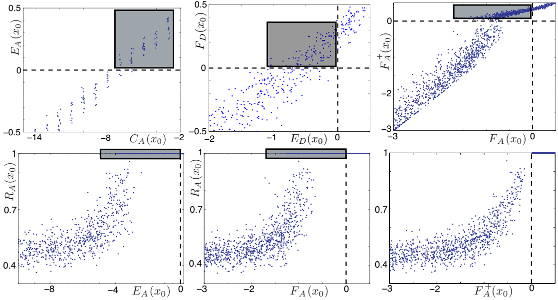
Figure 8: First row: pairwise comparison of identifiability criteria C , ERC , F and F^+ . The shaded rectangle on each plot delimits the vectors x_0 for which the criterion on the abscissa fails to recognize them as identifiable, whereas the criterion on the ordinate axis succeeds in identifying them. Second row: exact recovery success measure R_A as a function of each identifiability criterion. The shaded rectangles show those vectors that are positively tested as identifiable by the corresponding criterion.
