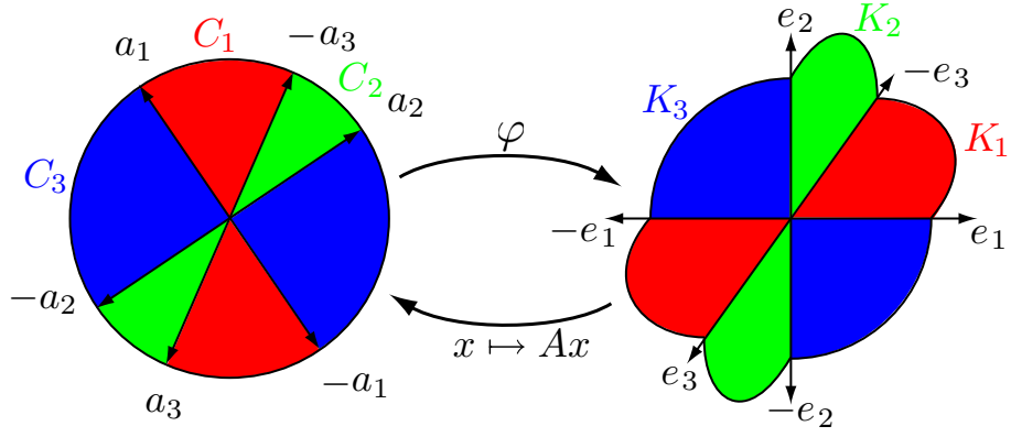
Figure 4: When n = 2 and p = 3 , the map \varphi acts as a bijection cone by cone and sends the unit disk onto a manifold of \mathbb{R}^3 .
