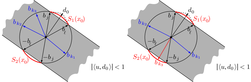
Figure 3: On the left, (S_1(x_0) \cup S_2(x_0)) \cap \mathcal{B} = \emptyset and then x_0 \in \mathcal{F} , on the right S_2(x_0) \cap \mathcal{B} \neq \emptyset and then x_0 \notin \mathcal{F} .
