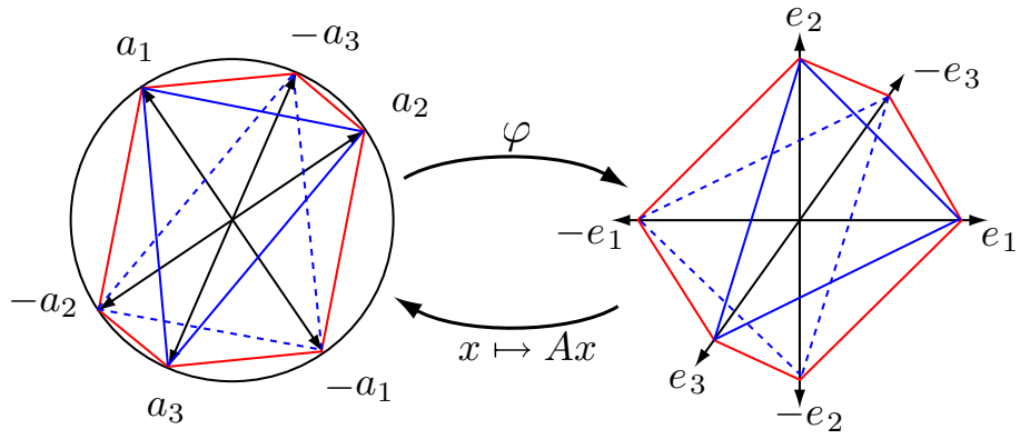
Figure 5: Right: The cones K_J \subset \mathcal{F} correspond to the edges, here in red, of the unit \ell_1 -ball. Left: The images by A of these edges are the (red) edges of the convex hull of the polytope (\pm a_j)_{j \leq p} .
