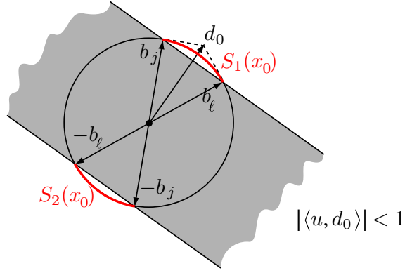
Figure 2: Example of vector d_0 and caps S_1(x_0) and S_2(x_0) for a vector x_0 \in K_{j,l} .
