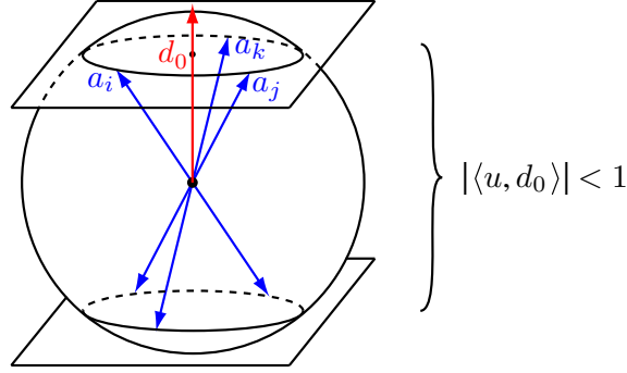
Figure 6: Example of 3D spherical caps associated to a vector x such that \|x\|_0 = 3 and x(i) > 0 , x(j) > 0 and x(k) > 0 .
