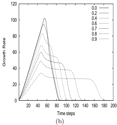
Figure 6: Growth curves of N(t) (a) and \Delta(t) (b) on a square grid for different anisotropic degrees \alpha .
