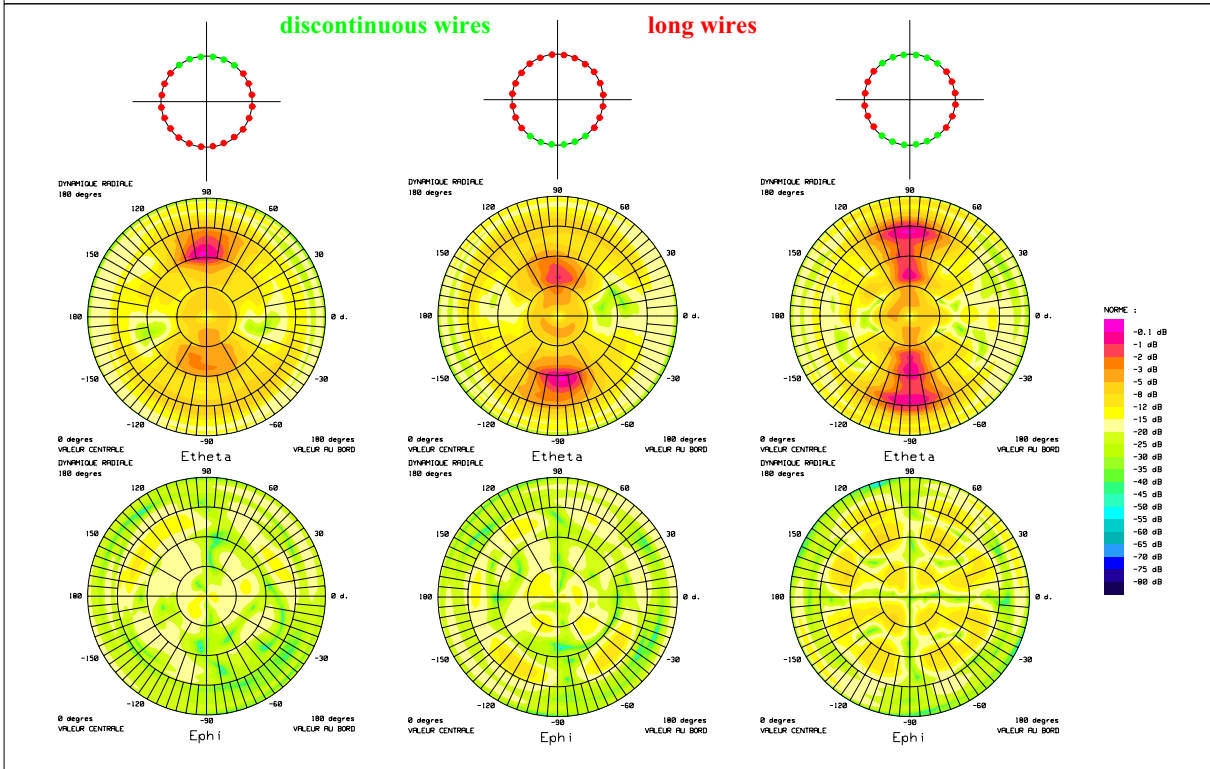
fig. 8: Measured radiation patterns of the technologic breadboard- F = 1.7 GHz
