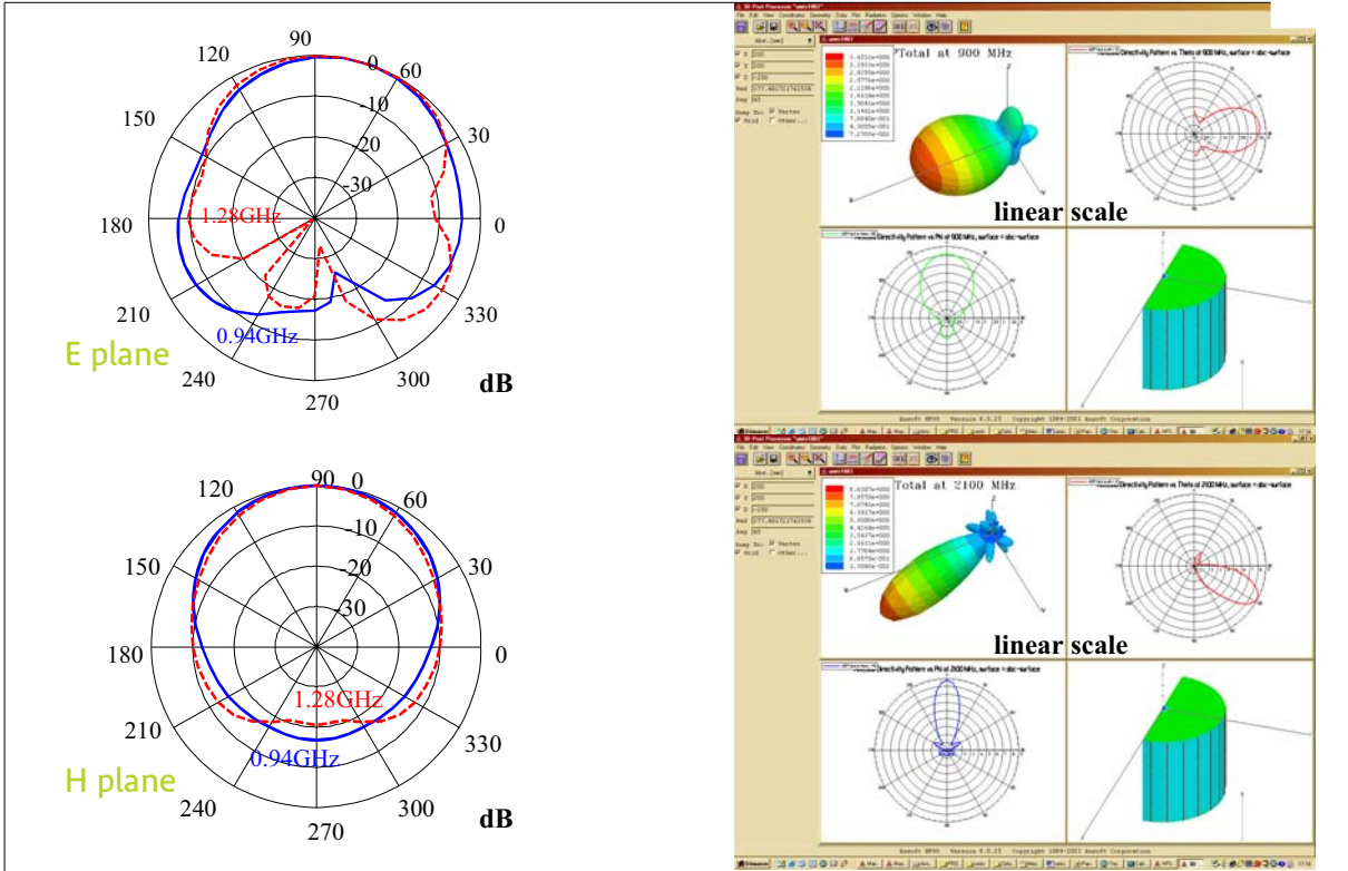
fig. 7: Simulated radiation patterns of the technologic breadboard
