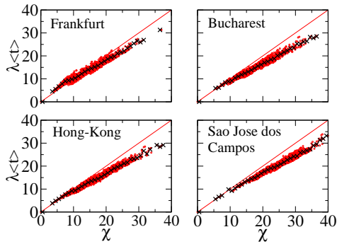
FIG. 4: (Color online) \lambda\langle t \rangle versus \chi on the WAN for diseases starting in different cities (whose name is specified in each graph). Each red circle corresponds to a city and averages are done over 1,000 realizations of the spreading. Crosses are an average over cities with the same \chi . When the initial seed is a hub, the average arrival time is larger than \chi in the first reached cities, due to the multiplicity of possible paths [22].
