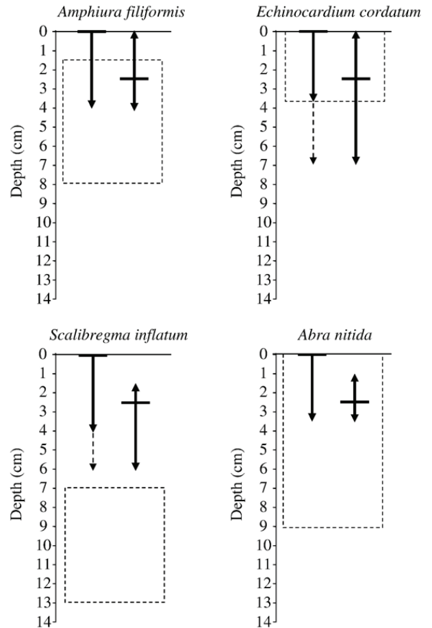
Fig. 1. Sediment zone (dotted rectangle) where individuals were found at the end of the experiment and range of luminophore movements (solid arrows) from surface (surface tracers) and 2.5 cm deep in the sediments (deep tracers) due to the four studied macrobenthic species ( A. filiformis , E. cordatum , S. inflatum and A. nitida ). Horizontal lines are the starting points for luminophores. Dotted arrows represent potentialities of tracer burying (i.e. potential deeper displacement of surface tracers according to the downward transport of deep tracers).
