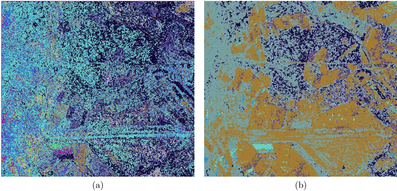
Figure 2: POL-SAR Wishart classification data of the master coherency [4620 × 4221 pixels]: (a) LAF, (b) ADAN estimated.
