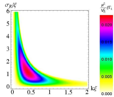
Figure 1: (color online) Density plot of the Lyapunov exponent of the BQPs for a 1D speckle potential.
