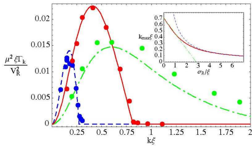
Figure 2: (color online) Lyapunov exponent of the BQPs for a 1D speckle potential. The lines correspond to Eq. (13) and the points to numerical results for \xi = 1.25 \times 10^{-5} L , V_R = 0.075\mu and \sigma_R = \sqrt{3/2}\xi (solid red line), \sigma_R = 3.7\xi (dashed blue line), \sigma_R = 0.4\xi (dash-dotted green line). Inset: localization maximum versus the ratio of the correlation length of the disorder to the healing length of the BEC (the dash-dotted and dashed lines correspond to the limits \sigma_R \ll \xi and \sigma_R \gg \xi respectively; see text).
