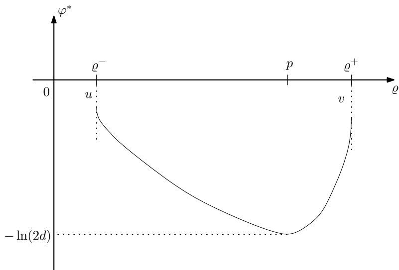
Figure 1: The function \varphi and its Legendre transform \varphi^*
