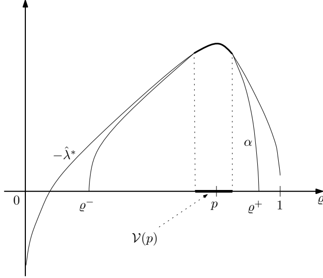
Figure 2: Typical behaviour of the function \alpha when d \geq 3
