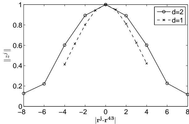
Figure 3: Crystal with a single defect: R = 0.15 , \eta^{43} = 1 and \theta^{inc} = \pi/2 . Cut of \|z^j\| along the axis going through \mathbf{r}^{43} with an angle \theta = \pi/6 .
