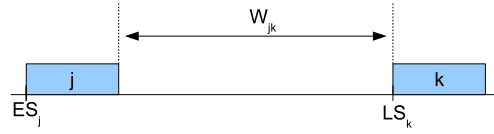
Fig. 3. Task insertion window
