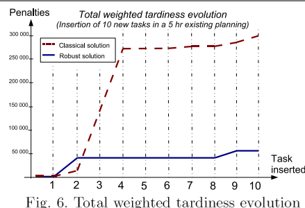
Fig. 6. Total weighted tardiness evolution
