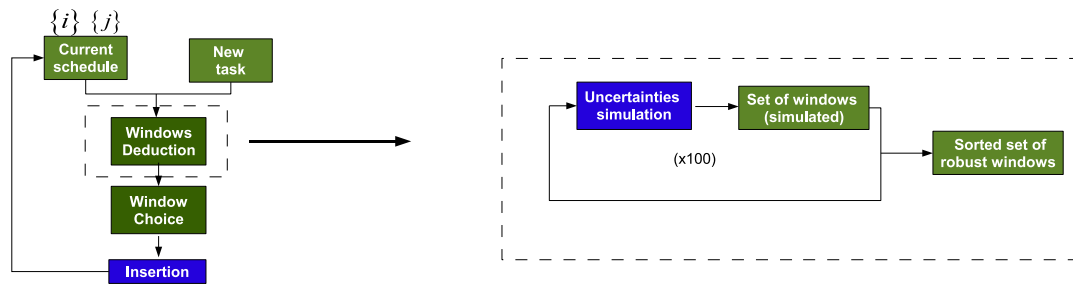
Fig. 4. Task insertion methode
